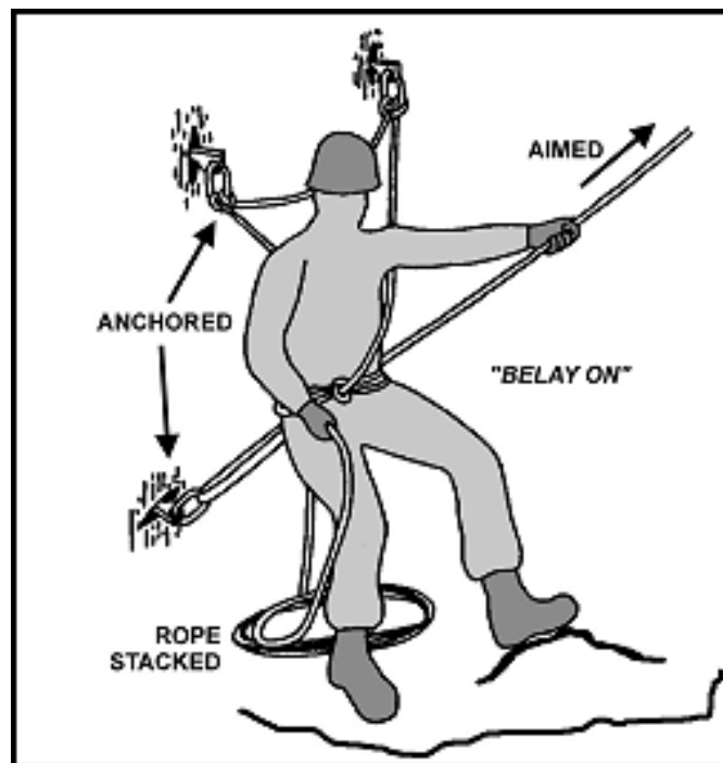
Figure 6-28. Belay setup.
