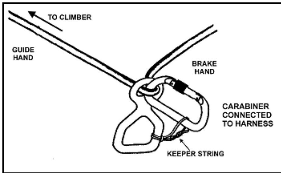
Figure 6-26. Figure-eight device.
