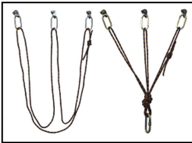
Figure 5-19. Pre-equalized anchor.
