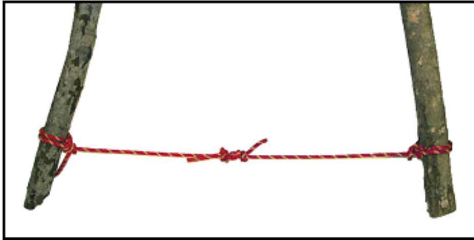
Figure 7-21. A-frame spreader.
