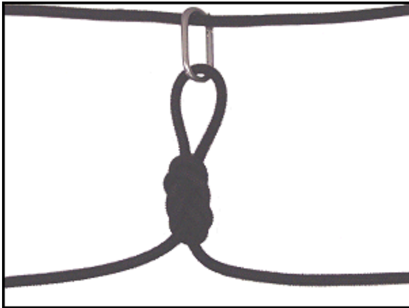
Figure 7-18. Hauling line.
