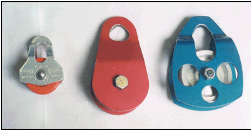
Figure 3-23. Pulley.
