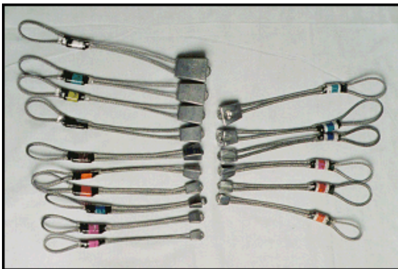
Figure 3-15. Chocks.
