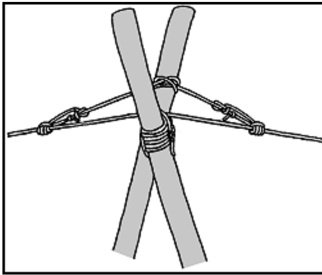
Figure 7-22. Anchoring the A-frame to the traverse rope.
