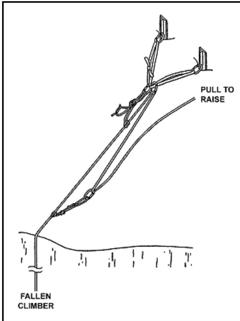
Figure 7-26. Z-pulley system.
