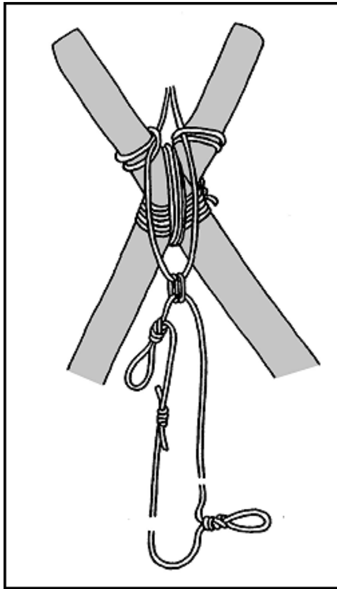
Figure 7-25. Attaching the anchor rope to the A-frame.
