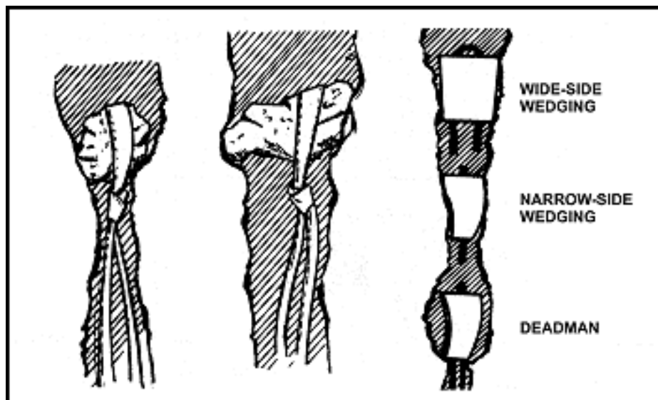
Figure 5-15. Chock placements.
