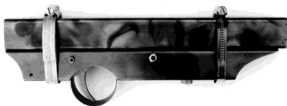
Photo 23: The receivers are clamped together with two hose clips.
