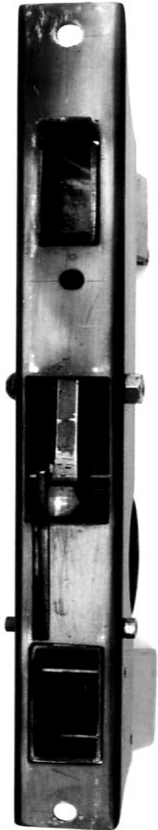
Photo 21: Top view of assembled receiver.
