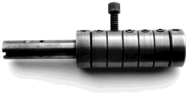
Photo 33: The fully assembled bolt. Note position of ejector slot in relation to bolt handle.
