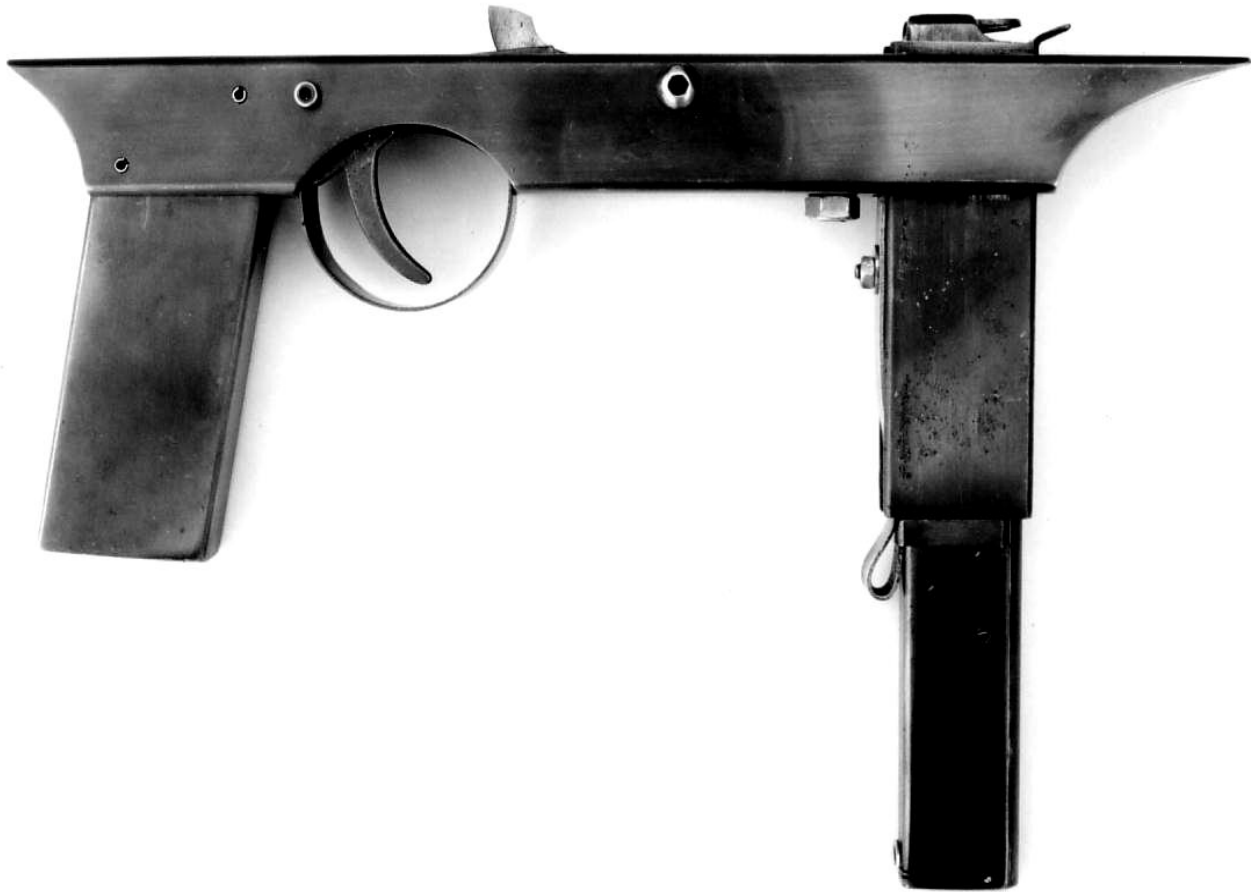
Photo 22: The fully assembled lower receiver.
