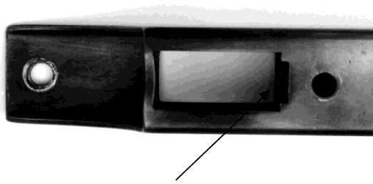
Photo 5: Lower magazine well recess Note shallow notch (arrowed).
