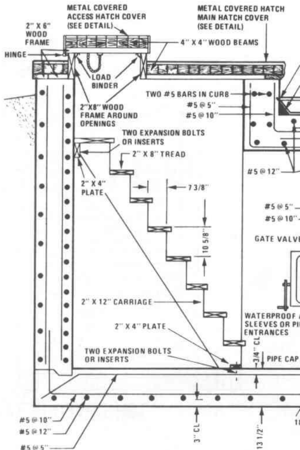
SECTION B-B
