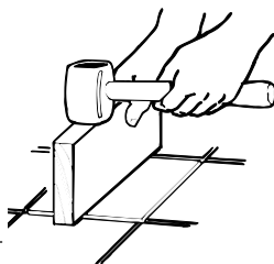
Fig 9. Tamp with mallet and wooden block.
