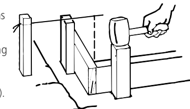
B. Position chalkline on corner stake. Adjust for drainage and mark line of stakes
